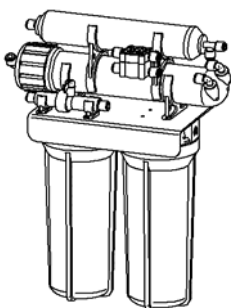
RO-050 manifold
